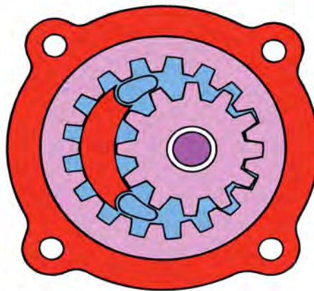
Internal gear pumps
