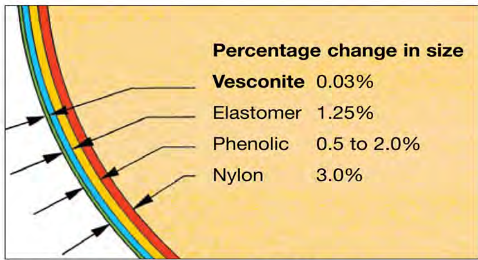
Swell of synthetic bearing materials due to water
