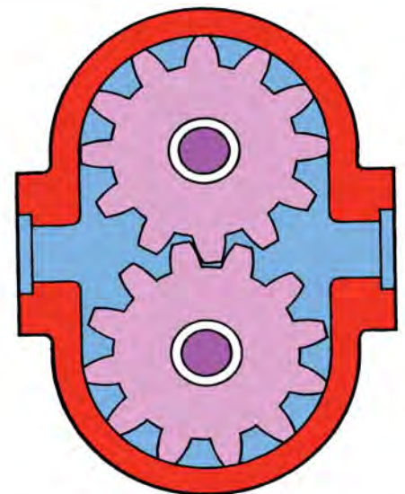
External gear pumps
